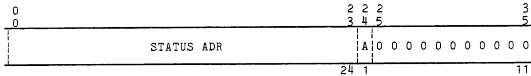
Figure 4-4. Bulk Store Data Control Block (DCB) Format, Word 1
