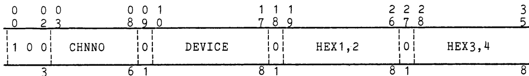
Figure 3-11. IOM Special Status Word Format
