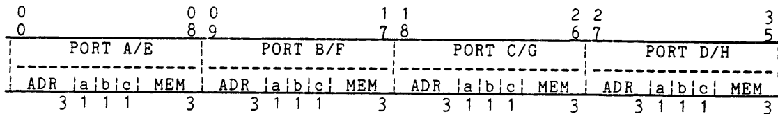
Figure 1-45. rsw xxxxx1/3 Data Format
