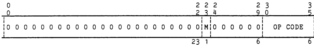
Figure 6-11. FNP Card Reader PCW Format
