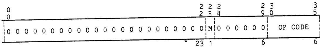
Figure 6-10. FNP Console PCW Format
