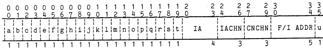
Figure 1-36. SCU Data Format, Word 1
