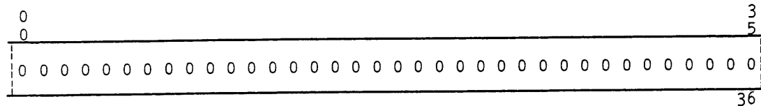
Figure 4-10. Bulk Store DCB Status Block Format, Word 3
