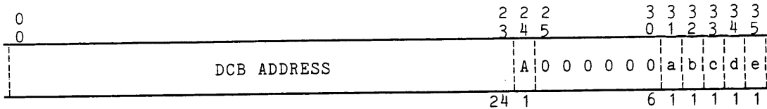
Figure 4-2. Bulk Store Current Status Block (CSB) Format, Word 0
