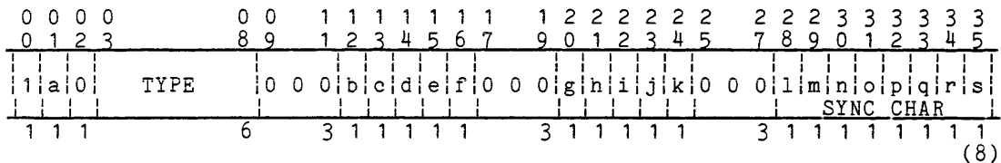
Figure 6-27. FNP HSLA Configuration Status Word Format
