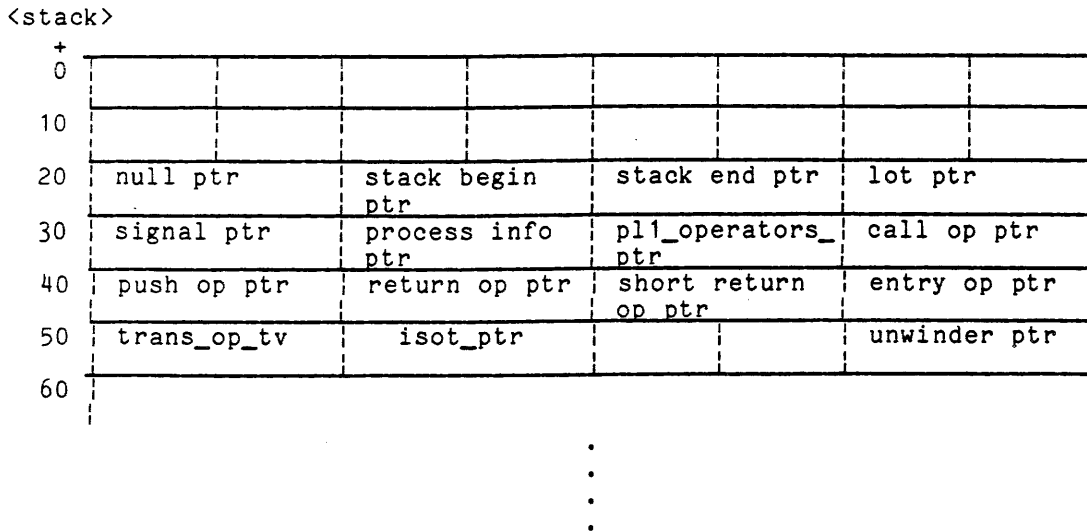
Figure 7-5. Stack Header Layout
