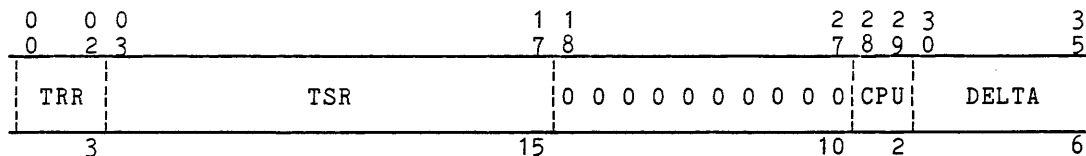
Figure 1-37. SCU Data Format, Word 2
