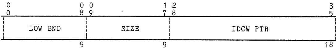
Figure 3-3. IOM List Pointer Word (LPW) Format
