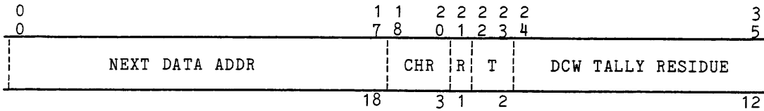
Figure 3-10. IOM Channel Status Data Format
