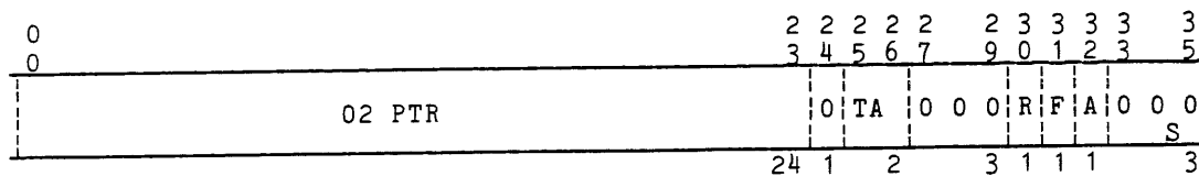
Figure 1-27. DU Pointers and Lengths Format, Word 4
