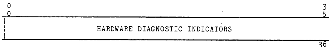
Figure 4-11. Bulk Store DCB Status Block Format, Word 4
