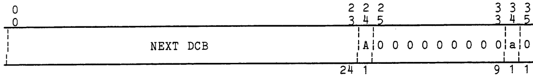
Figure 4-3. Bulk Store Data Control Block (DCB) Format, Word 0
