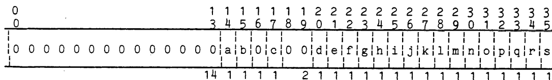
Figure 6-9. FNP DIA Status Word Format
