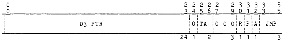
Figure 1-29. DU Pointers and Lengths Format, Word 6
