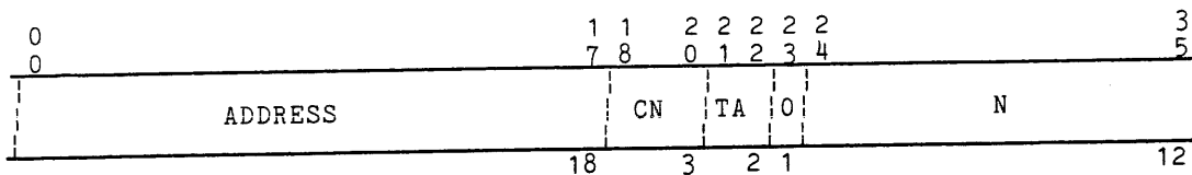
Figure 1-15. EIS Alphanumeric Data Descriptor Format
