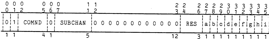
Figure 6-20. FNP HSLA PCW1 Format
