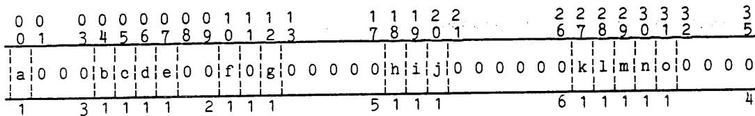
Figure 6-15. FNP LSLA Active Status Word Format
