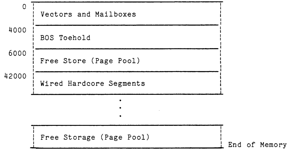
Figure 7-3. Main Memory Map for Multics Service
