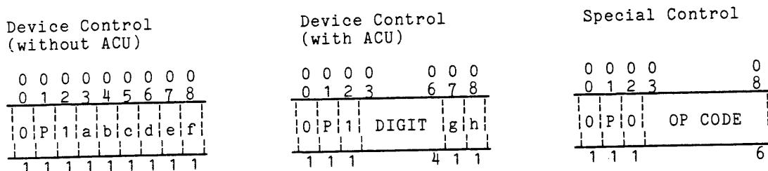
Figure 6-17. FNP LSLA Device Control Characters
