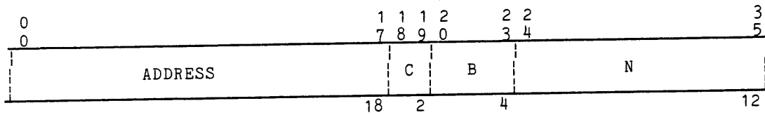
Figure 1-14. EIS Bit String Data Descriptor Format
