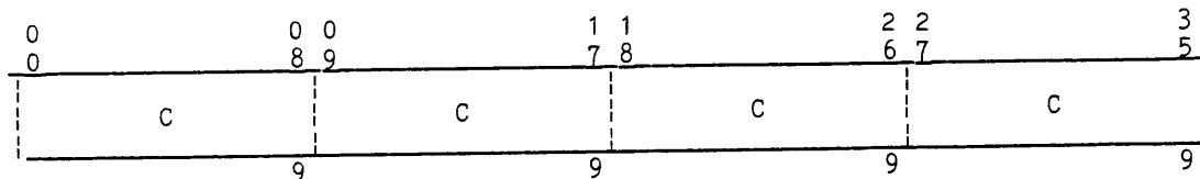
Figure 1-20. EIS Alphanumeric Data Format, 9-bit Mode
