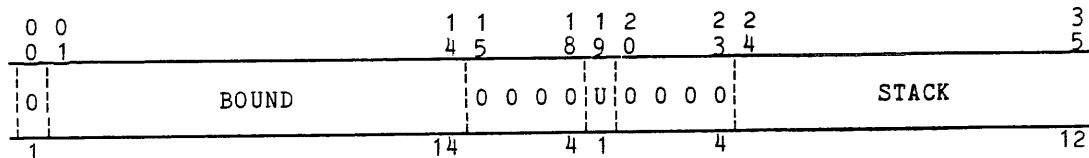
Figure 1-6. Descriptor Base Register (DBR) Format
