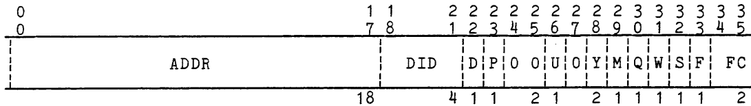
Figure 1-5. Page Table Word (PTW) Format
