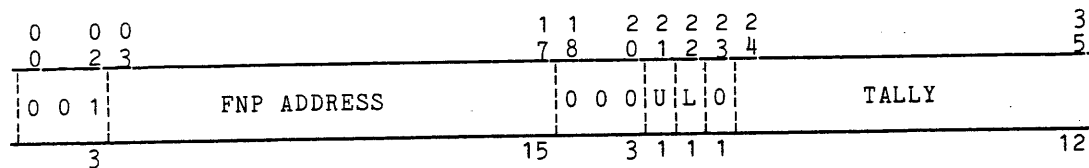
Figure 6-8. FNP DIA DCW Format
