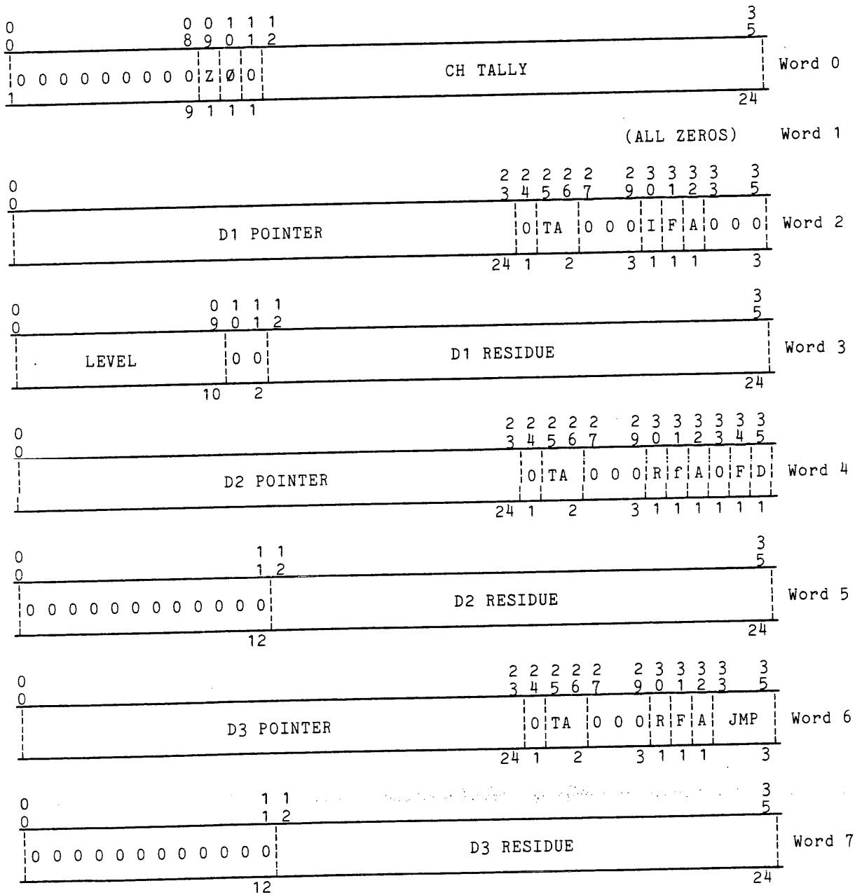
Figure B-5. DU Pointers and Lengths Format
