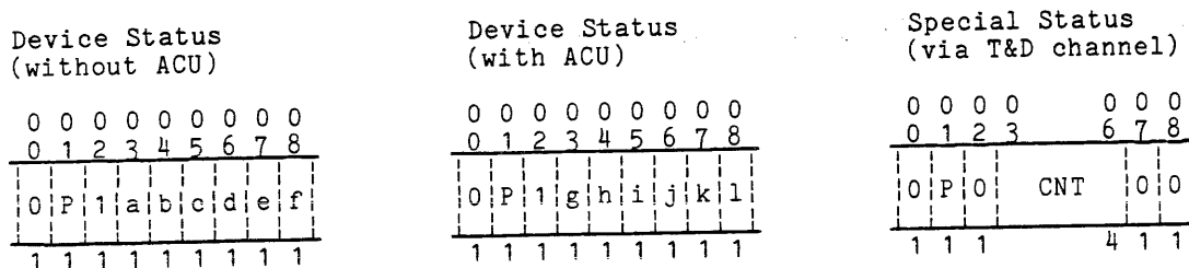
Figure 6-18. FNP LSLA Device Status Character Formats
