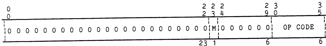
Figure 6-12. FNP Line Printer PCW Format
