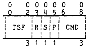
Figure 6-24. FNP HSLA CCC Format
