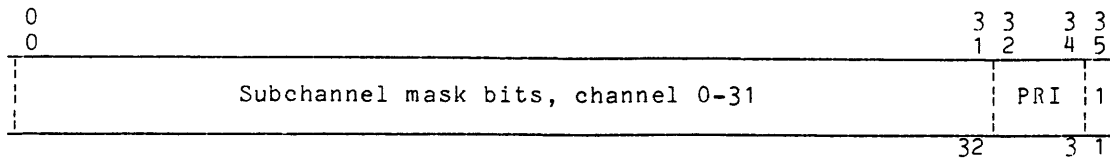
Figure 6-25. FNP HSLA Mask Register Word Format
