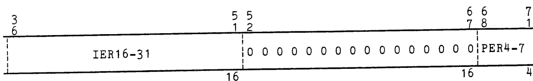
Figure 2-2. Interrupt Mask Register (rscr/sscr 000N2X) Data Format
