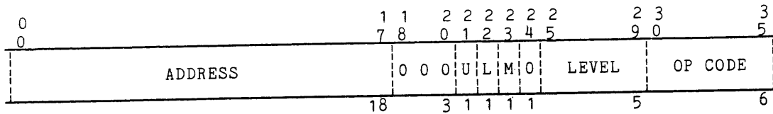
Figure 6-7. FNP DIA PCW Format
