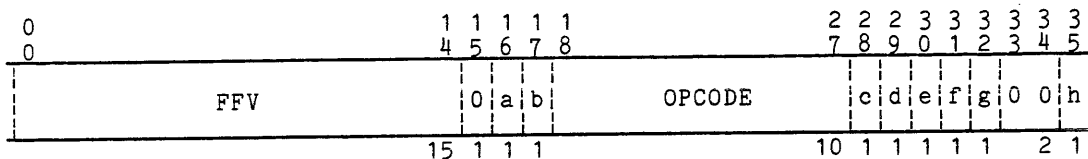
Figure 1-47. Mode Register Format
