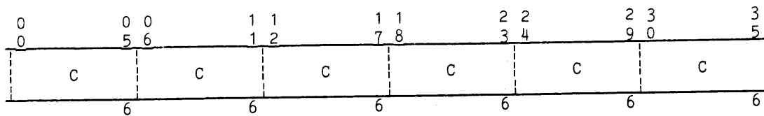
Figure 1-19. EIS Alphanumeric Data Format, 6-bit Mode
