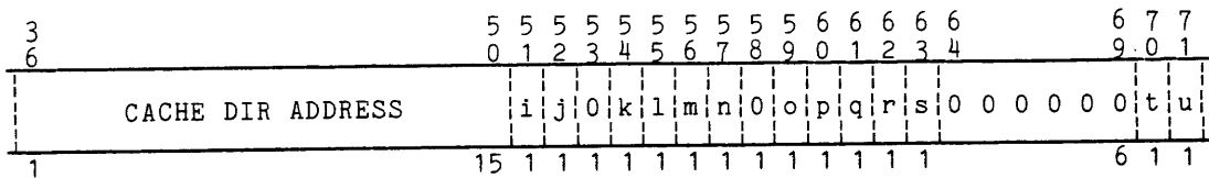
Figure 1-48. Cache Mode Register Format
