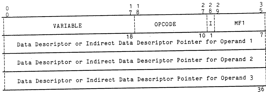
Figure 1-11. EIS Multiword Instruction Format
