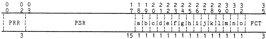
Figure 1-35. SCU Data Format, Word 0
