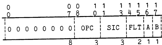
Figure 6-5. FNP IOM Fault Status Word Format
