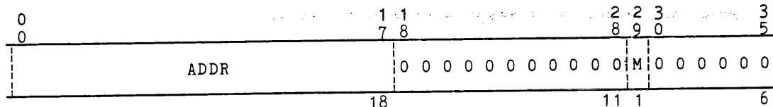
Figure 1-9. PTW Associative Memory (PTWAM) Register Format
