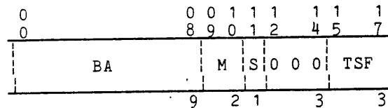
Figure 6-23. FNP HSLA BAW Format
