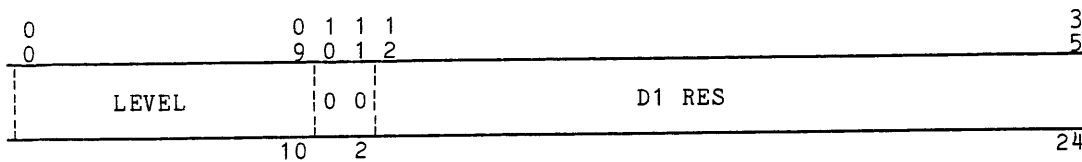
Figure 1-26. DU Pointers and Lengths Format, Word 3
