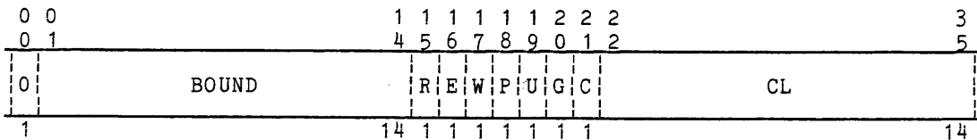
Figure 1-4. Segment Descriptor Word (SDW) Format
