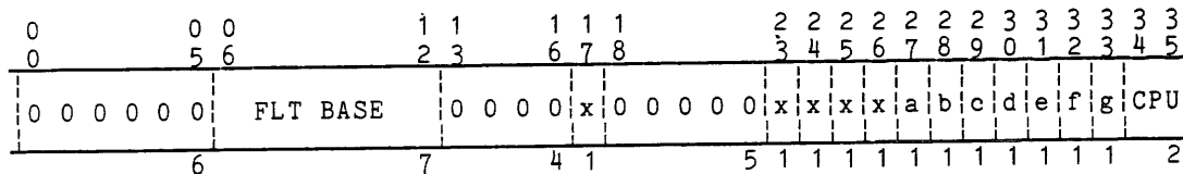
Figure 1-44. rsw xxxxx2 Data Format
