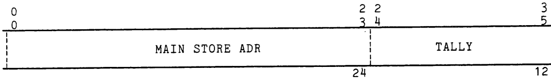
Figure 4-5. Bulk Store Data Control Block (DCB) Format, Word 2
