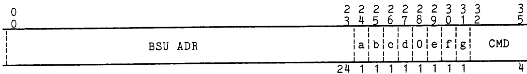
Figure 4-6. Bulk Store Data Control Block (DCB) Format, Word 3
