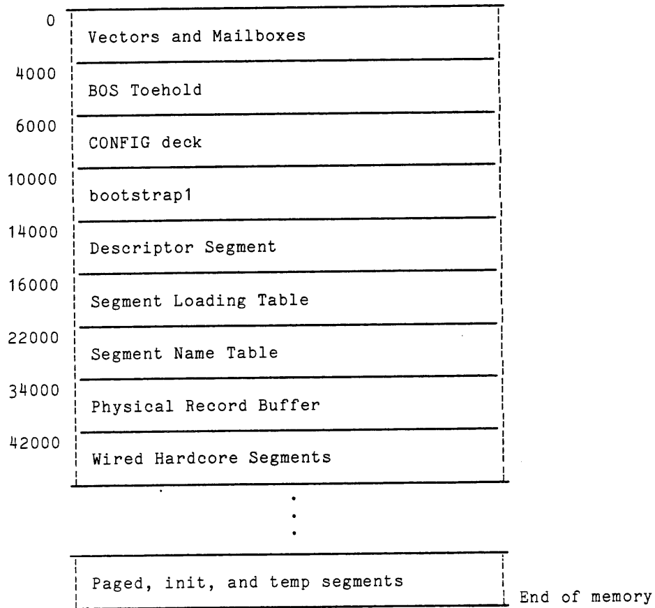
Figure 7-2. Main Memory Map for Bootstrap1
