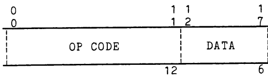
Figure 6-3. FNP Nonstore Reference Instruction Format - Group 2
