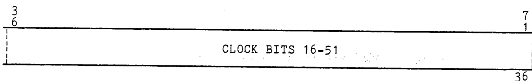
Figure 2-4. System Clock (rscr/sscr/rccl 00004X) Data Format
