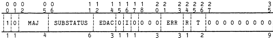
Figure 4-7. Bulk Store DC3 Status Block Format, Word 0
