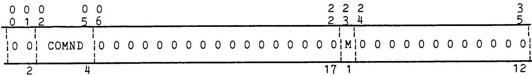
Figure 6-13. FNP LSLA PCW0 Format
