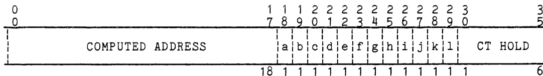
Figure 1-40. SCU Data Format, Word 5
