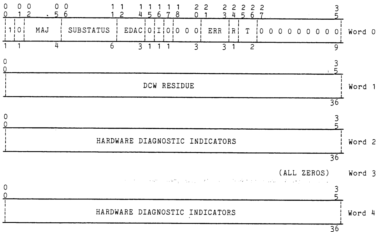
Figure B-3. Bulk Store DCB Status Block Format
