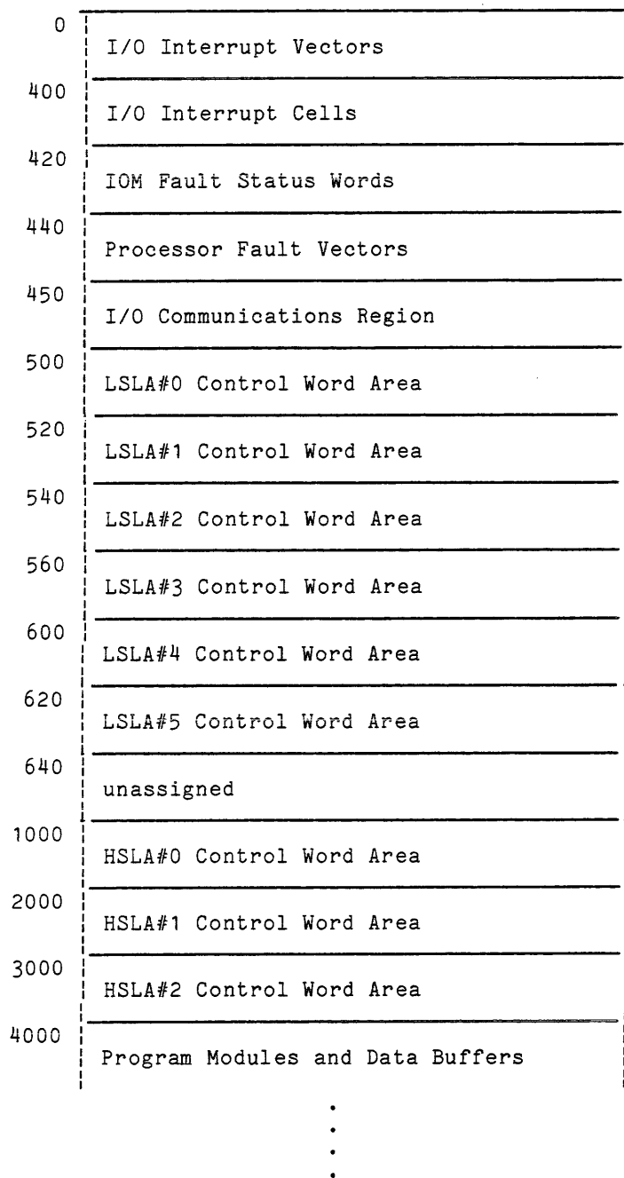
Figure 6-28. FNP Store Map
