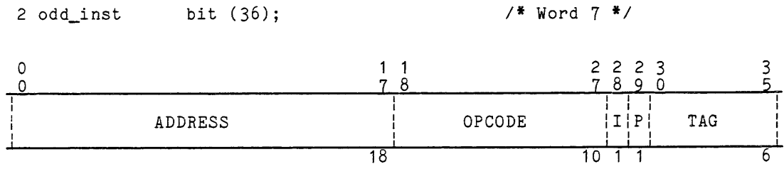
Figure 1-42. SCU Data Format, Word 7
