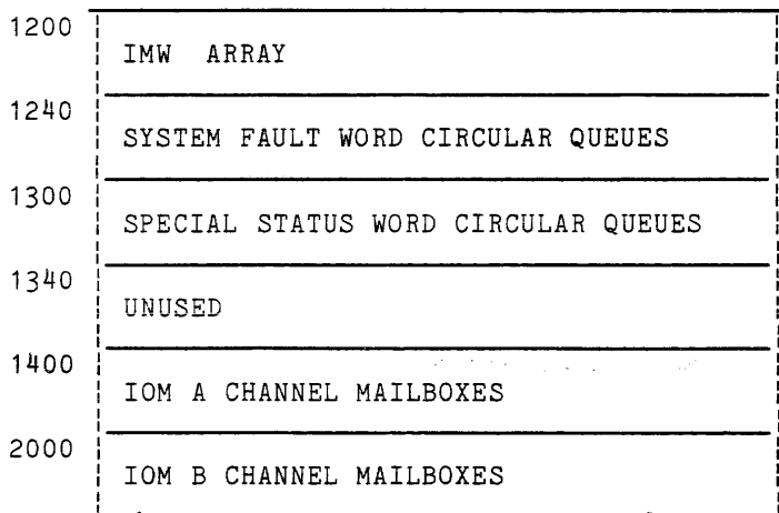
Figure 3-1. IOM Mailbox Layout
