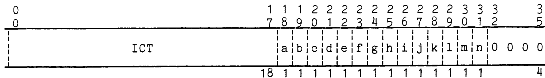
Figure 1-39. SCU Data Format, Word 4
