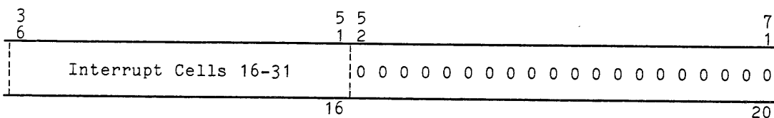
Figure 2-3. Interrupt Cells (rscr/sscr 00003X) Data Format
