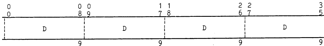
Figure 1-22. EIS Numeric Data Format, 9-Bit Mode
