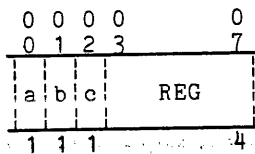
Figure 1-12. EIS Data Descriptor Modification Field (MF) Format
