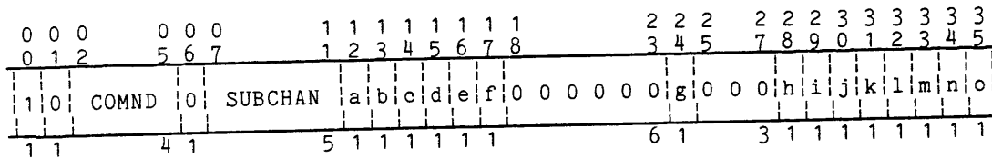
Figure 6-21. FNP HSLA PCW2 Format
