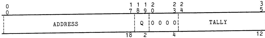
Figure 3-8. IOM Status Control Word (SCW) Format
