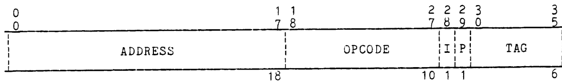
Figure 1-41. SCU Data Format, Word 6
