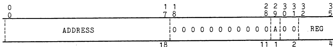
Figure 1-13. EIS Indirect Data Descriptor Pointer Format
