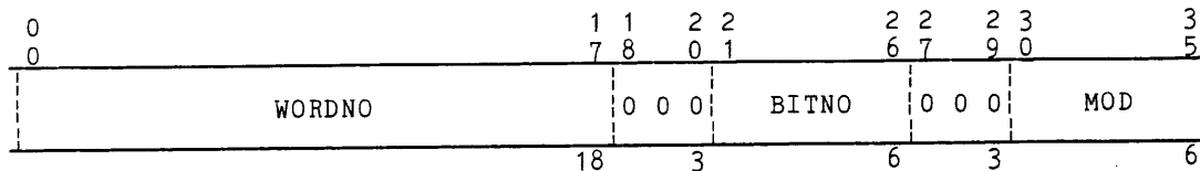
Figure 1-3. ITP Pair Format
