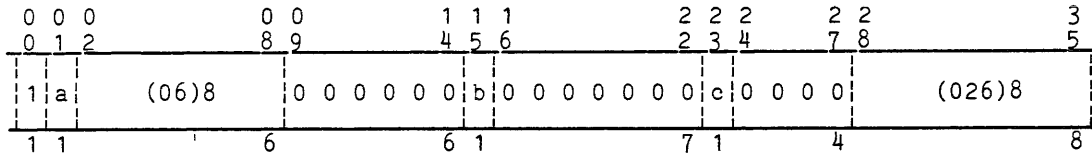
Figure 6-16. FNP LSLA Configuration Status Word
