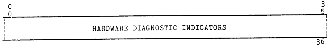
Figure 4-9. Bulk Store DCB Status Block Format, Word 2
