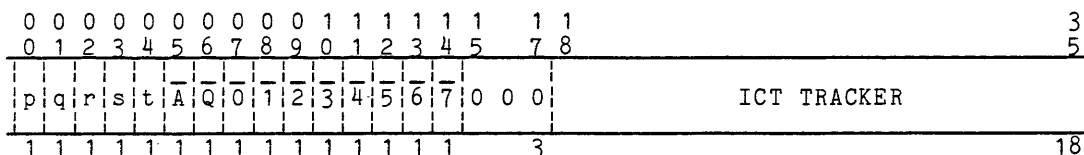
Figure 1-32. OU History Register Format
