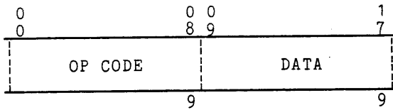
Figure 6-2. FNP Nonstore Reference Instruction Format - Group 1
