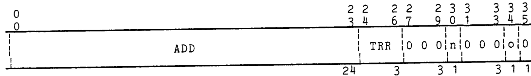
Figure 1-33. APU History Register Format
