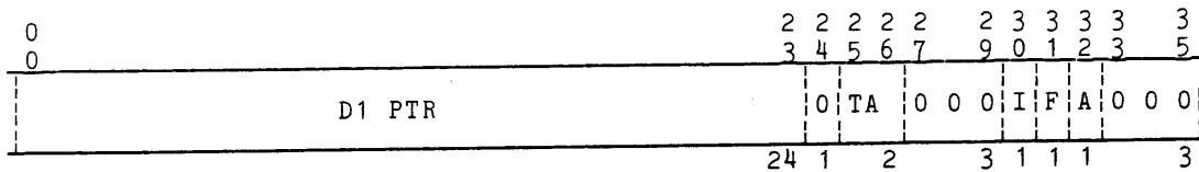
Figure 1-25. DU Pointers and Lengths Format, Word 2
