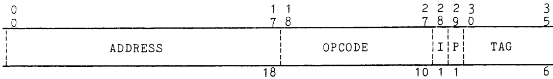
Figure 1-1. Basic Instruction Word Format
