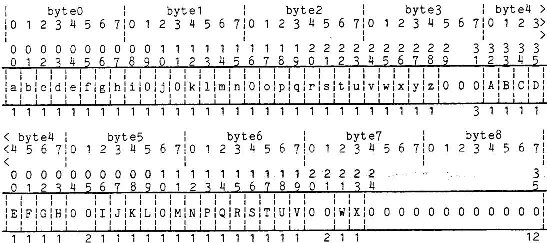
Figure C-3. DSS190B Extended Status
