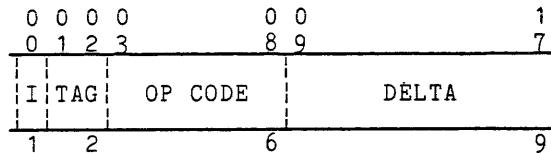
Figure 6-1. FNP Store Reference Instruction Format
