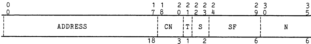
Figure 1-16. EIS Numeric Data Descriptor Format
