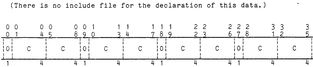
Figure 1-18. EIS Alphanumeric Data Format, 4-bit Mode
