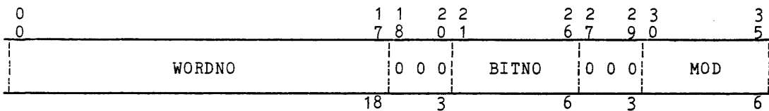
Figure 1-2. ITS Pair Format
