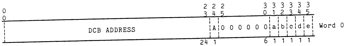
Figure B-4. Bulk Store Current Status Block (CSB) Format
