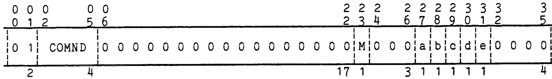
Figure 6-14. FNP LSLA PCW1 Format
