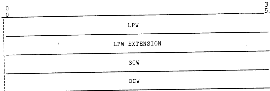
Figure 3-2. IOM Channel Mailbox Layout
