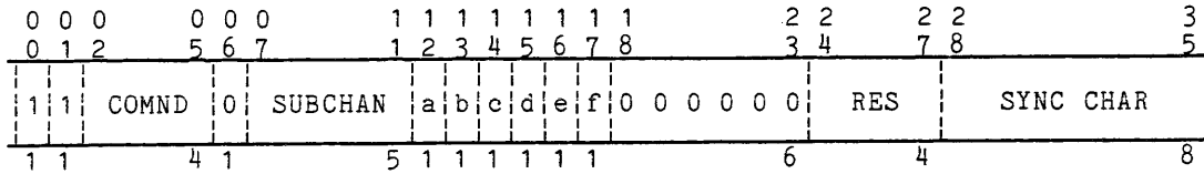
Figure 6-22. FNP HSLA PCW3 Format
