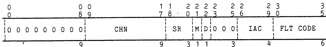
Figure 3-9. IOM System Fault Status Word Format
