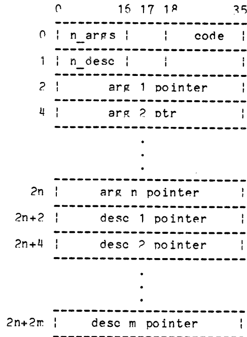
Figure 7-7. Argument List Layout For Call Without Environment Pointer
