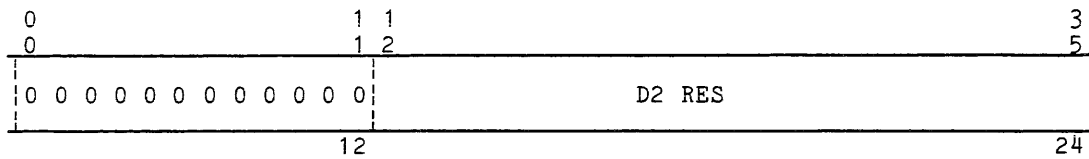
Figure 1-28. DU Pointers and Lengths Format, Word 5
