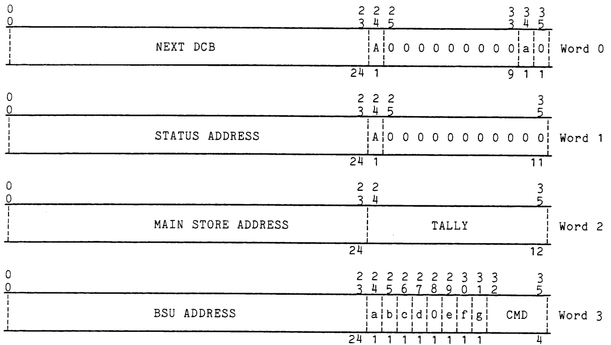
Figure B-2. Bulk Store Data Control Block (DCB) Format
