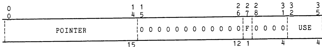
Figure 1-8. SDW Associative Memory (SDWAM) Match Logic Register Format
