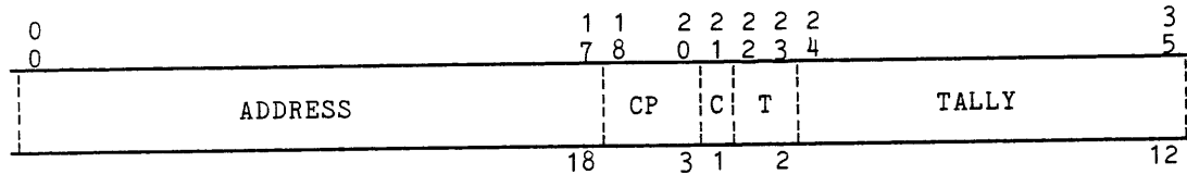
Figure 3-5. IOM Data Transmission DCW Format
