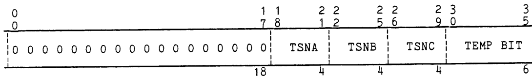
Figure 1-38. SCU Data Format, Word 3
