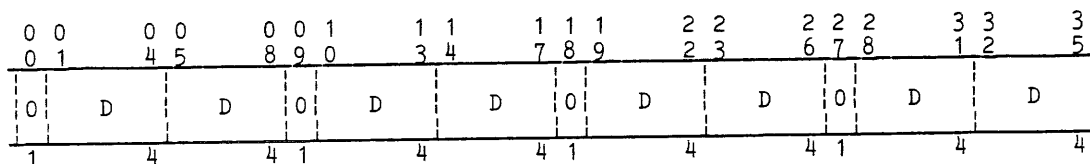
Figure 1-21. EIS Numeric Data Format, 4-Bit Mode
