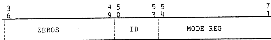
Figure 2-1. Controller Mode Register (rscr/sscr 00000X) Data Format
