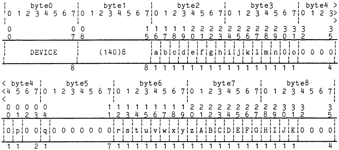
Figure C-1. DSS181 Extended Status
