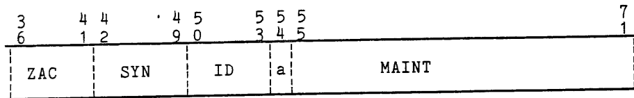
Figure 2-5. Store Mode Register (rscr/sscr 00006X) Data Format
