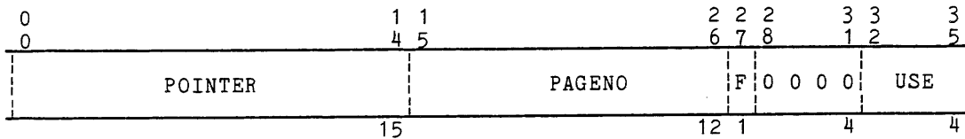
Figure 1-10. PTW Associative Memory (PTWAM) Match Logic Register Format
