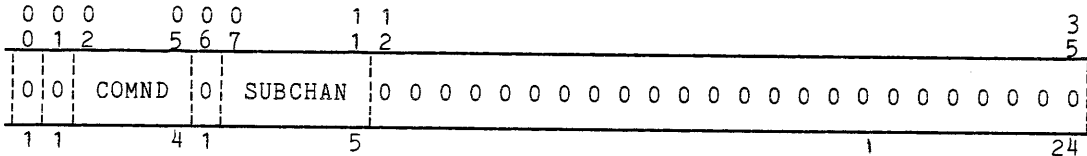
Figure 6-19. FNP HSLA PCW0 Format
