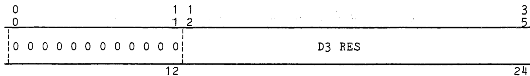
Figure 1-30. DU Pointers and Lengths Format, Word 7
