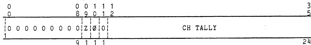
Figure 1-23. DU Pointers and Lengths Format, Word 0
